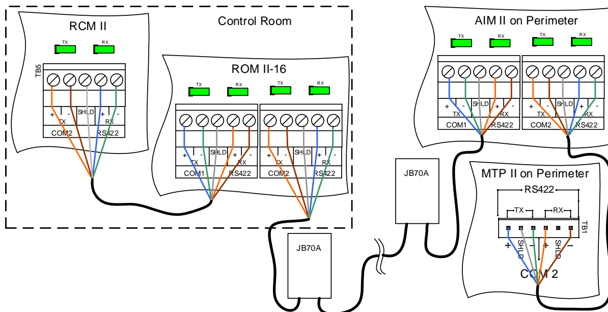
Figure 3 –ROM II Communications Wiring Diagram
